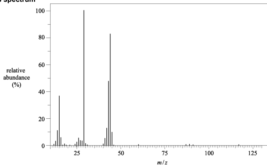
Mass spectrum
