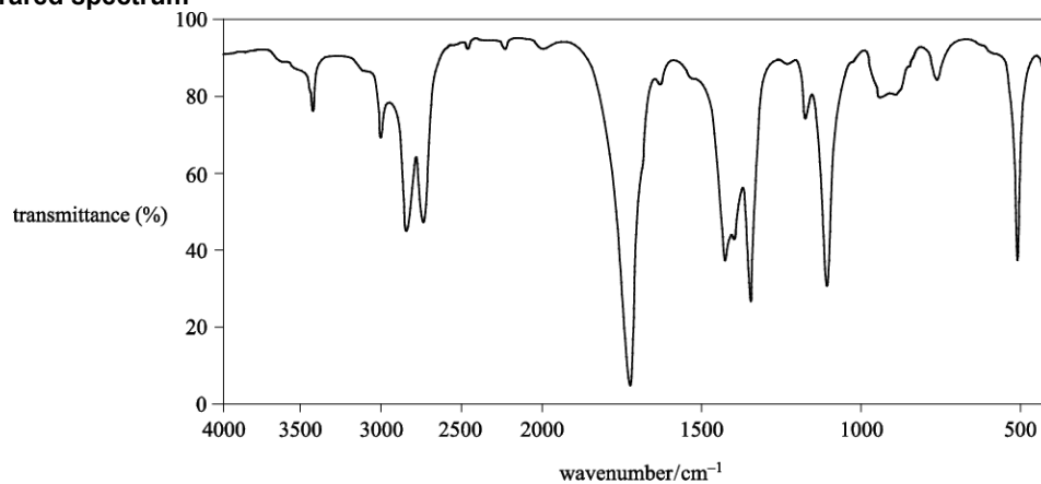
Infrared spectrum
